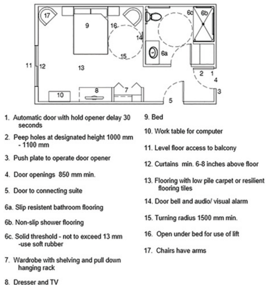
Figure H: Single queen bed room layout
