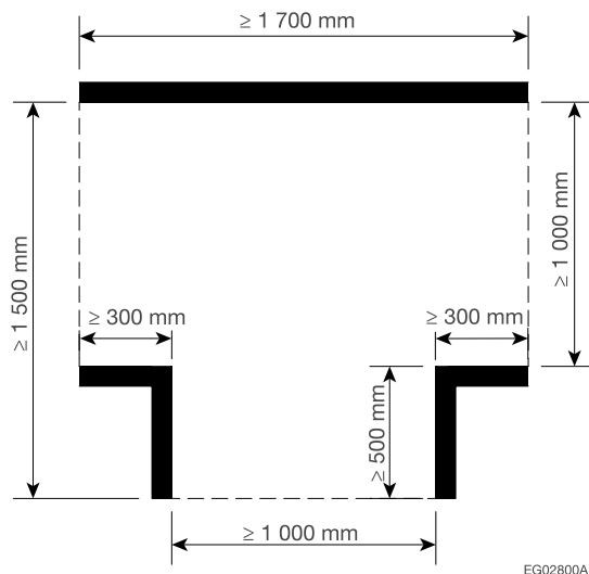
Figure A-3.8.3.2.(6) above from the NBC(AE) – T-shaped wheelchair turning space
