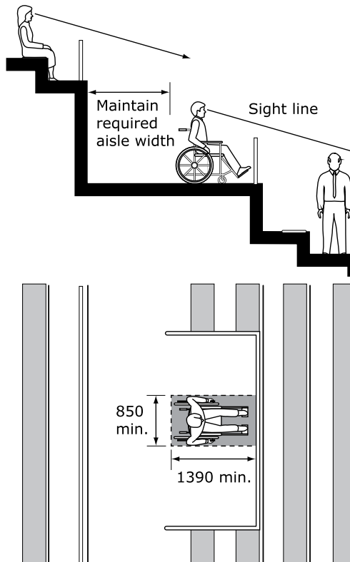
Figure 59 above from CSA B651 – Reserved viewing spaces in a place of assembly (See Clause 6.7.3.3.)
