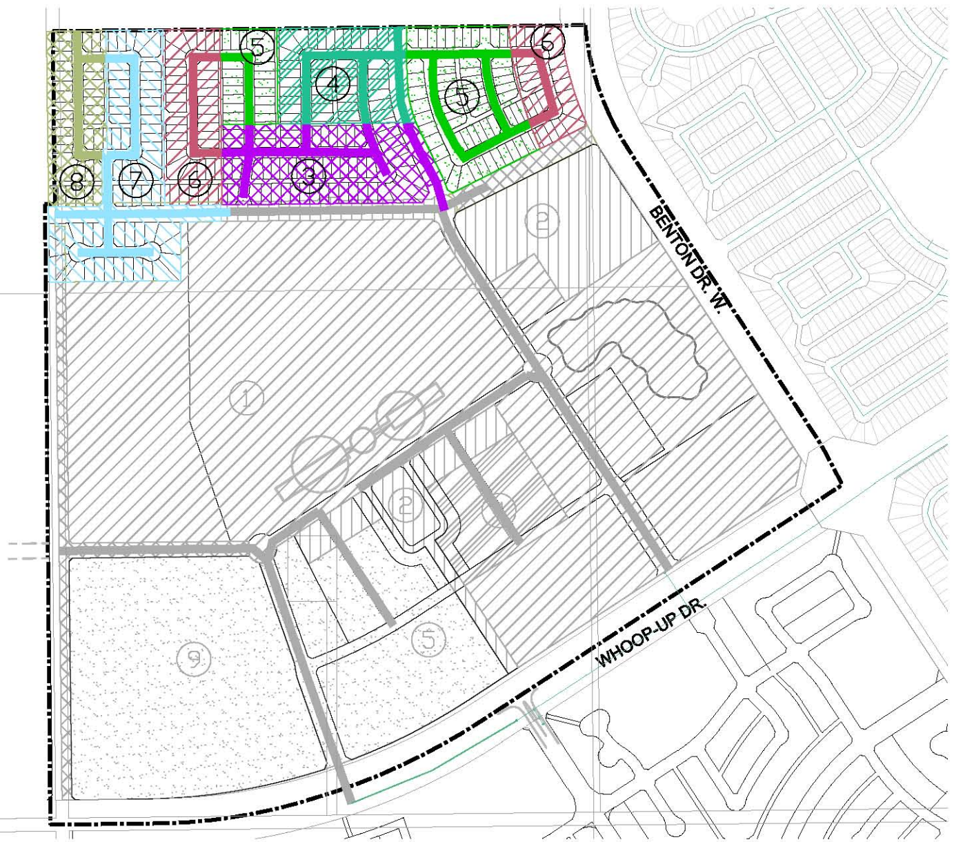
Figure 9 Sanitary Service Staging
