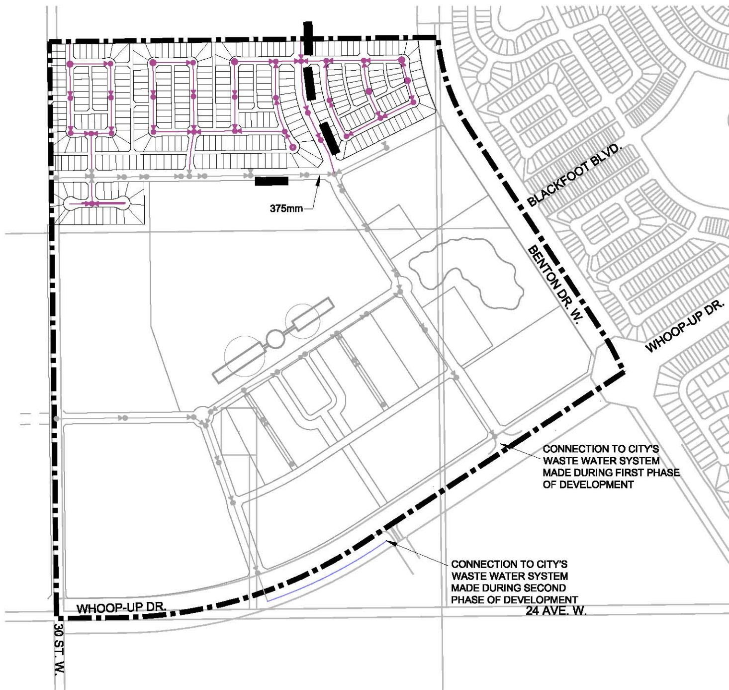
Figure 8 Sanitary Servicing Concept
